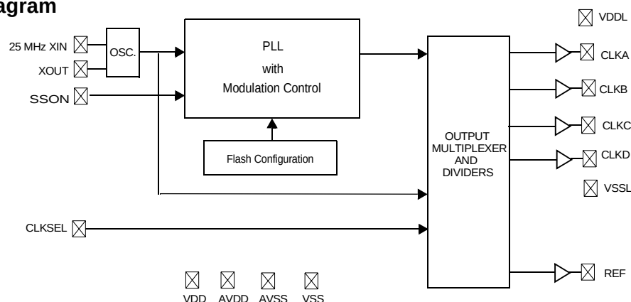
CY26121 16-pin TSSOP
