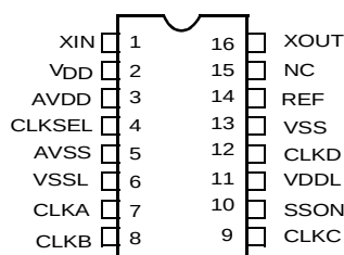
CY26121 16-pin TSSOP
