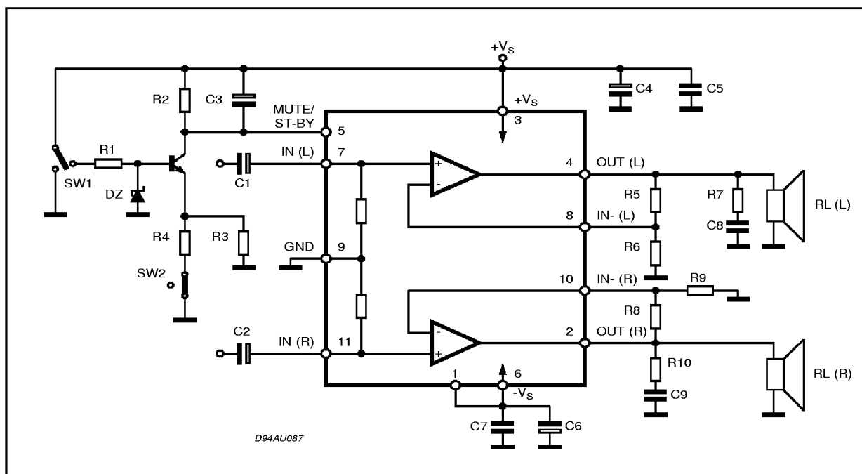
Figure 4: Test and Application Circuit (Stereo Configuration).
