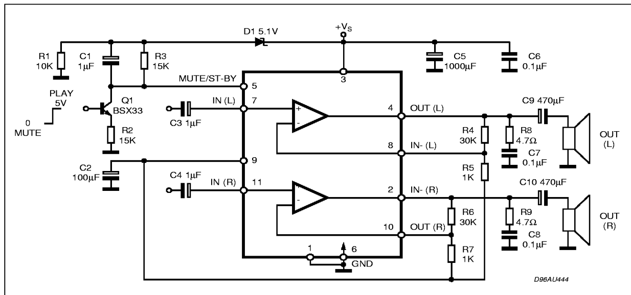
Figure 2: Single Supply Application
