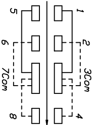
CIRCUIT: DP3T
