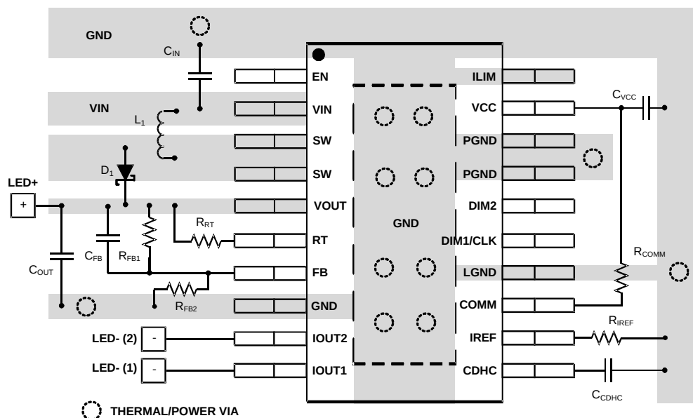
Figure 32. Layout Recommendation
