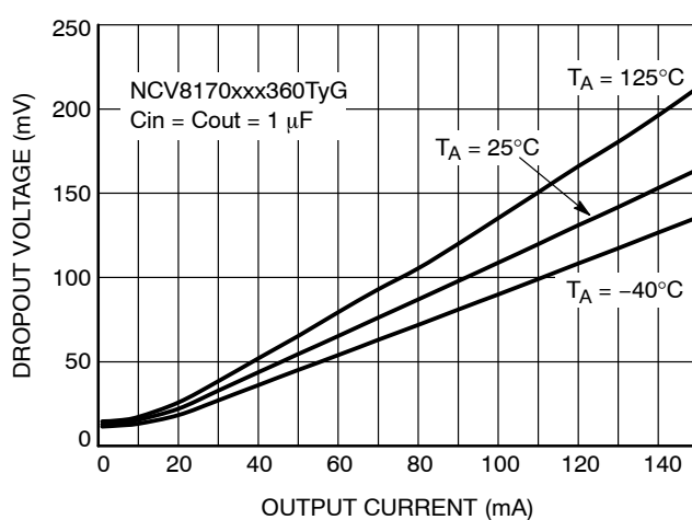
Figure 14. Dropout Voltage vs. Output Current, Vout = 3.6 V
