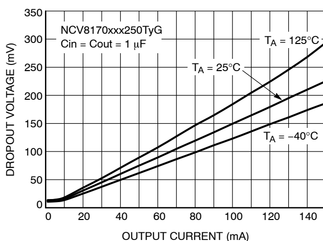
Figure 12. Dropout Voltage vs. Output Current, Vout = 2.5 V
