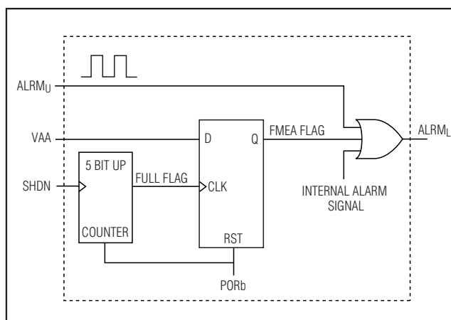
Figure 18. Internal FMEA \overline{\text{SHDN}} Pin Functionality Circuit
