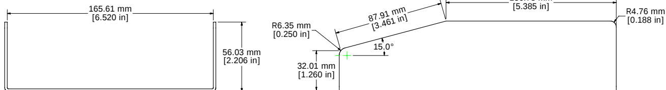
ASSEMBLY - END VIEW (OPEN)
