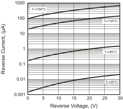
Fig.2 - Leakage Current
