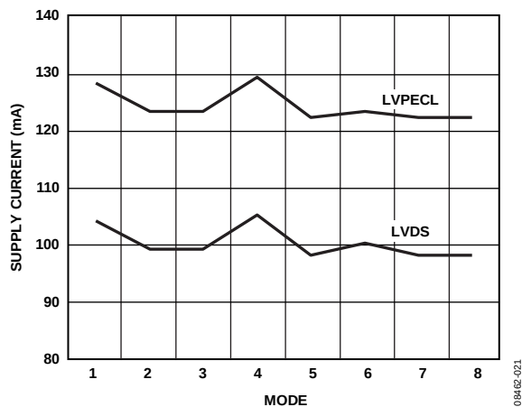
Figure 13. Typical Supply Current vs. Mode (see Table 12)
