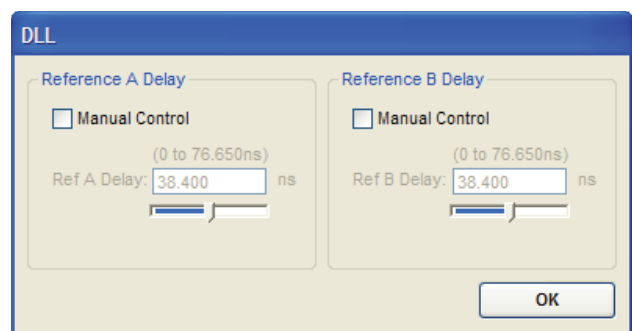
Figure 11. DLL Window
