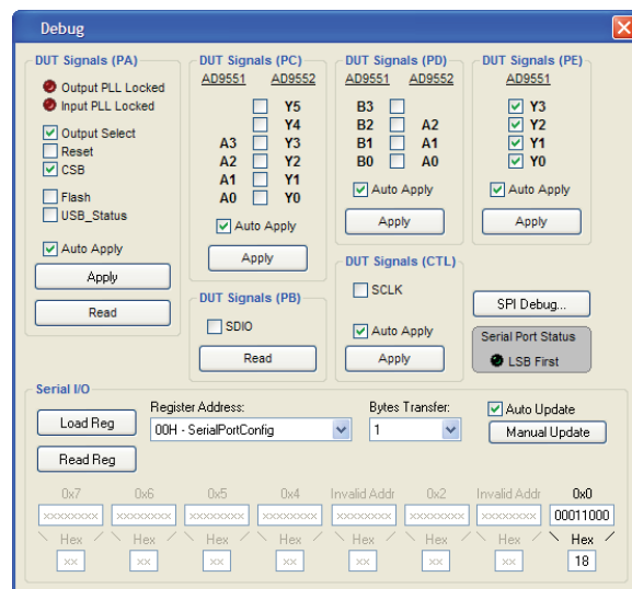
Figure 7. Debug Window
