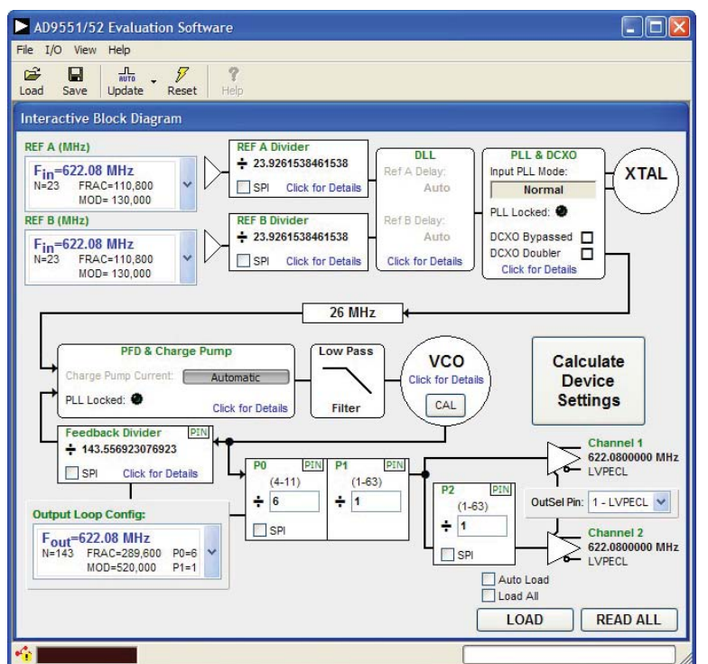
Figure 4. AD9551 Evaluation Software Main Window
