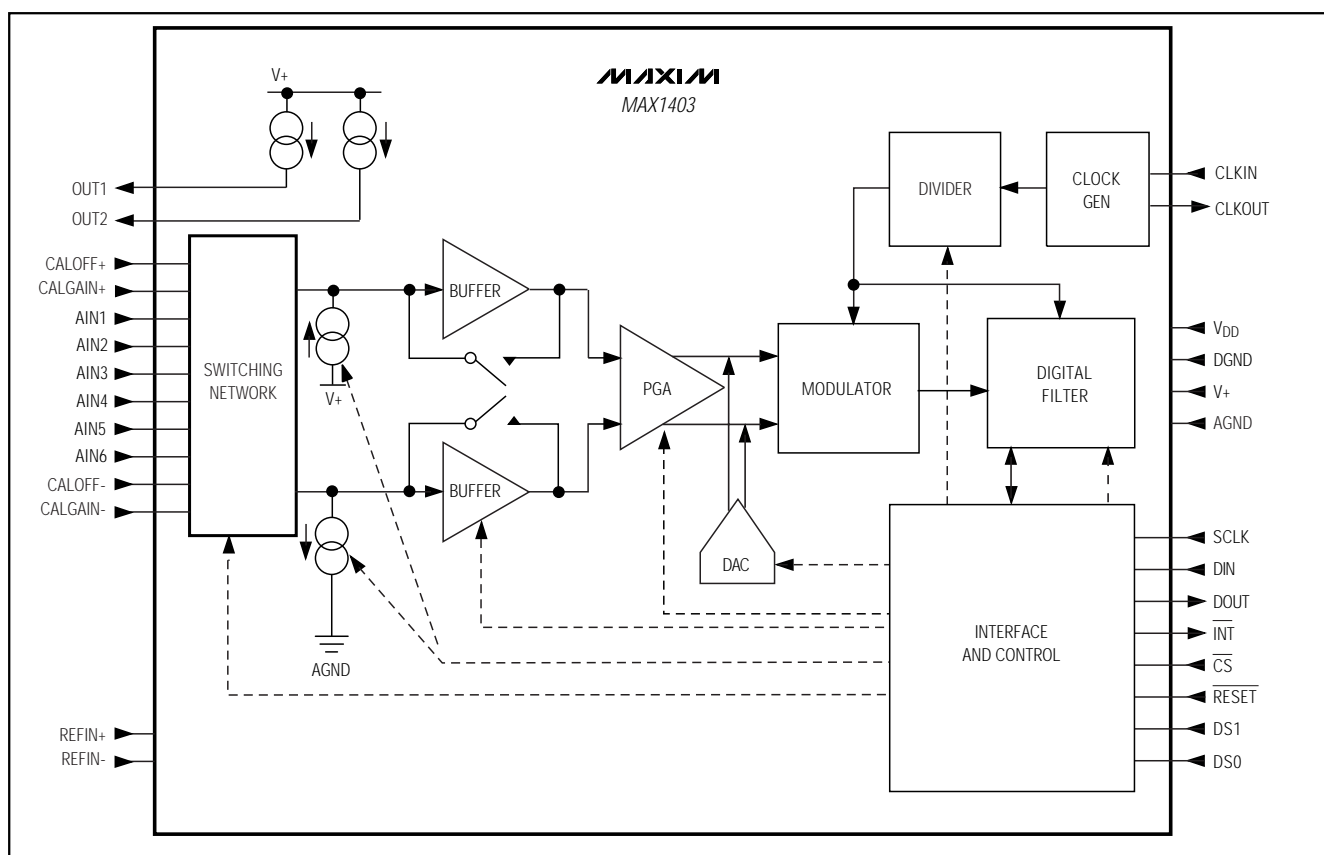
Figure 2. Functional Diagram
