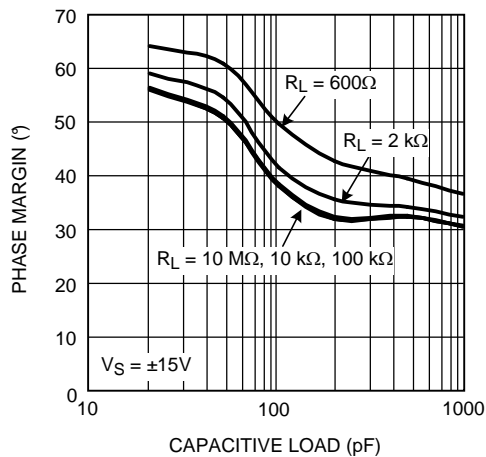
Figure 45. Phase Margin vs. Capacitive Load
