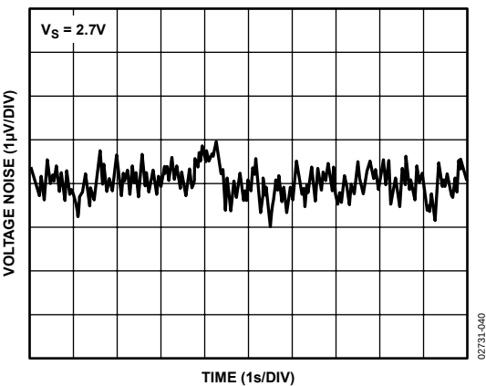
Figure 40. 0.1 Hz to 10 Hz Input Voltage Noise
