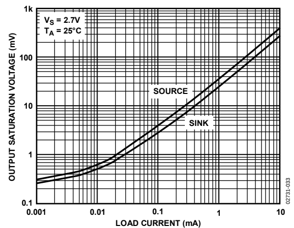
Figure 33. Output Saturation Voltage vs. Load Current
