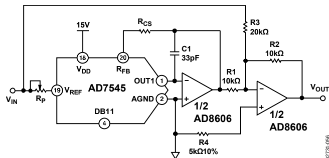
Figure 56. Bipolar Operation
