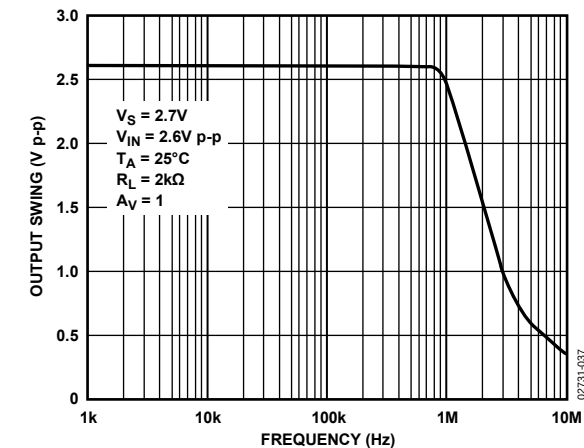
Figure 37. Closed-Loop Output Voltage Swing vs. Frequency
