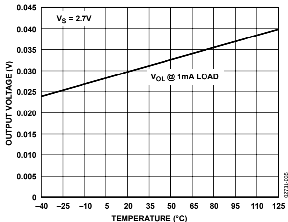
Figure 35. Output Voltage Swing vs. Temperature
