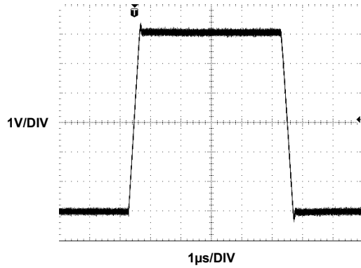
FIGURE 19. LARGE SIGNAL TRANSIENT RESPONSE
