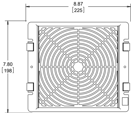
TEP6 EXHAUST GRILLE
