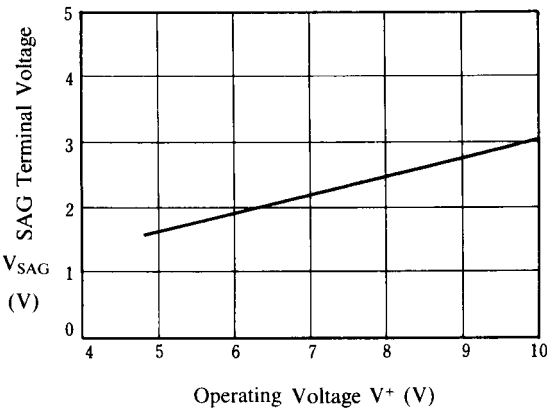
SAG Terminal Voltage vs. Operating Voltage (Ta = 25°C)
