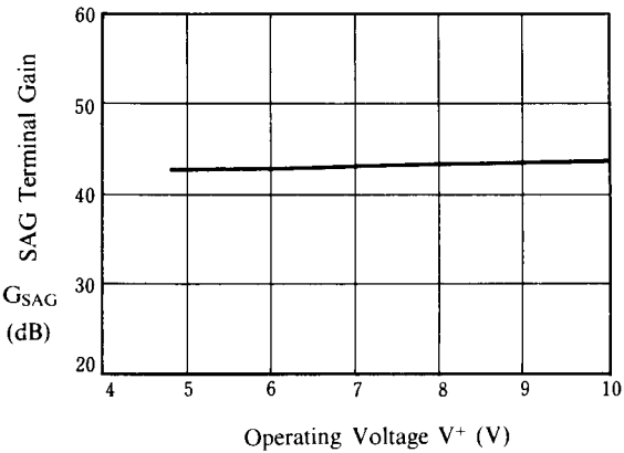
SAG Terminal Gain vs. Operating Voltage (Ta = 25°C)
