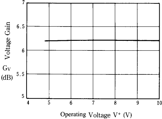
Voltage Gain vs. Operating Voltage (Ta = 25°C, 1V P-P , 1MHz sinewave signal input)
