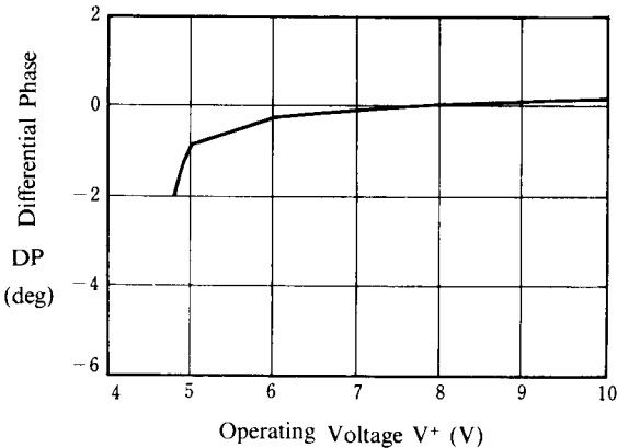
Differential Phase vs. Operating Voltage (Ta = 25°C, 1V P-P staircase signal input)
