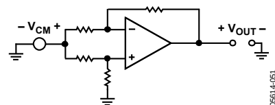
Figure 44. Common-Range Subtractor
