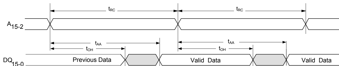
Figure 5. Read Cycle Timing 1 ( \overline{CE} LOW, \overline{OE} LOW)
