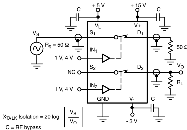
Figure 4. Crosstalk
