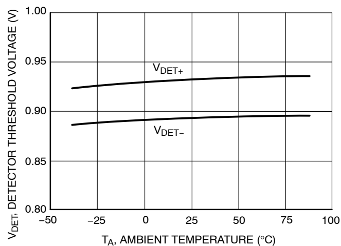
Figure 6. NCP300/1 Series 0.9 V Detector Threshold Voltage versus Temperature
