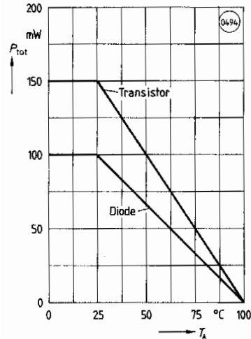
Figure 18. Permissible power dissipation transistor and diode P_{tot}=f(T_A)
