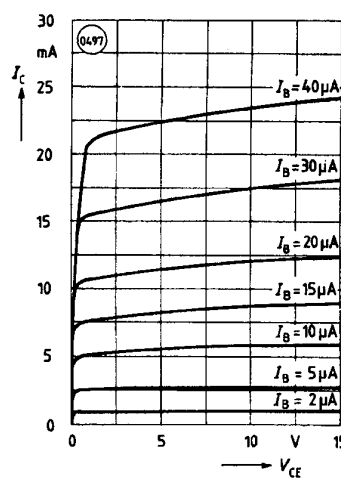
Figure 10. Output characteristics CNY17-3, -4 ( T_A=25^\circ\text{C} ) I_C=f(V_{CE})
