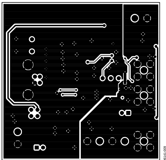
Figure 11. EVAL-AD5063EB—Solder-Side Artwork
