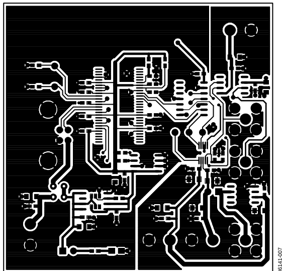
Figure 10. EVAL-AD5063EB —Component Side Artwork
