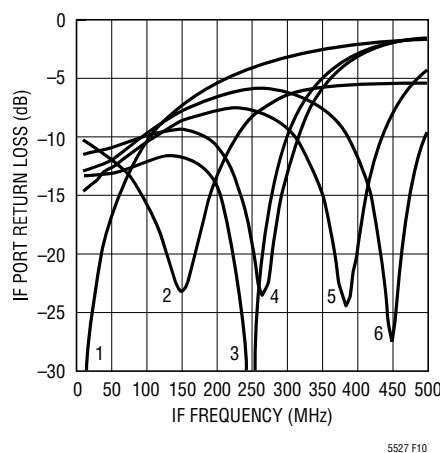
Figure 10. IF Output Return Losses with Lowpass/Transformer Matching
