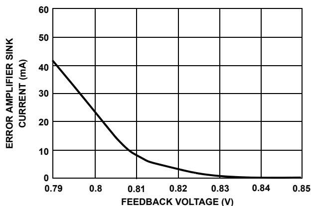
FIGURE 43. LINEAR CONTROLLER GAIN
