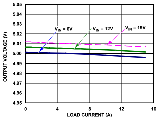
FIGURE 2. PWM1 LOAD REGULATION
