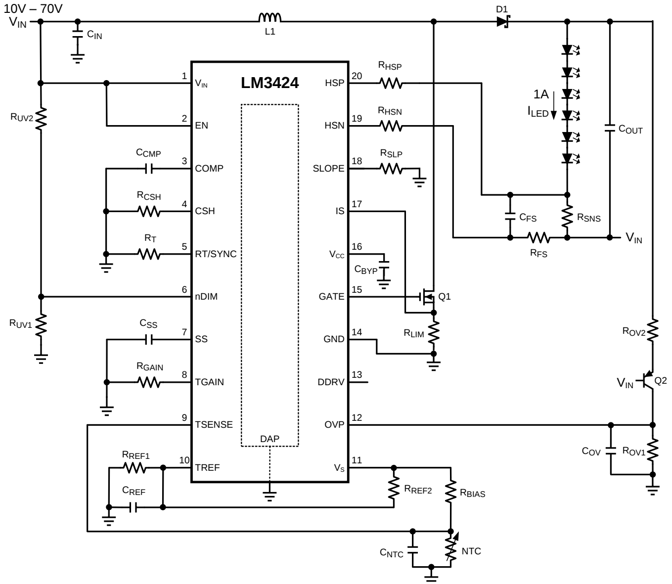
Figure 39. Buck-Boost Application
