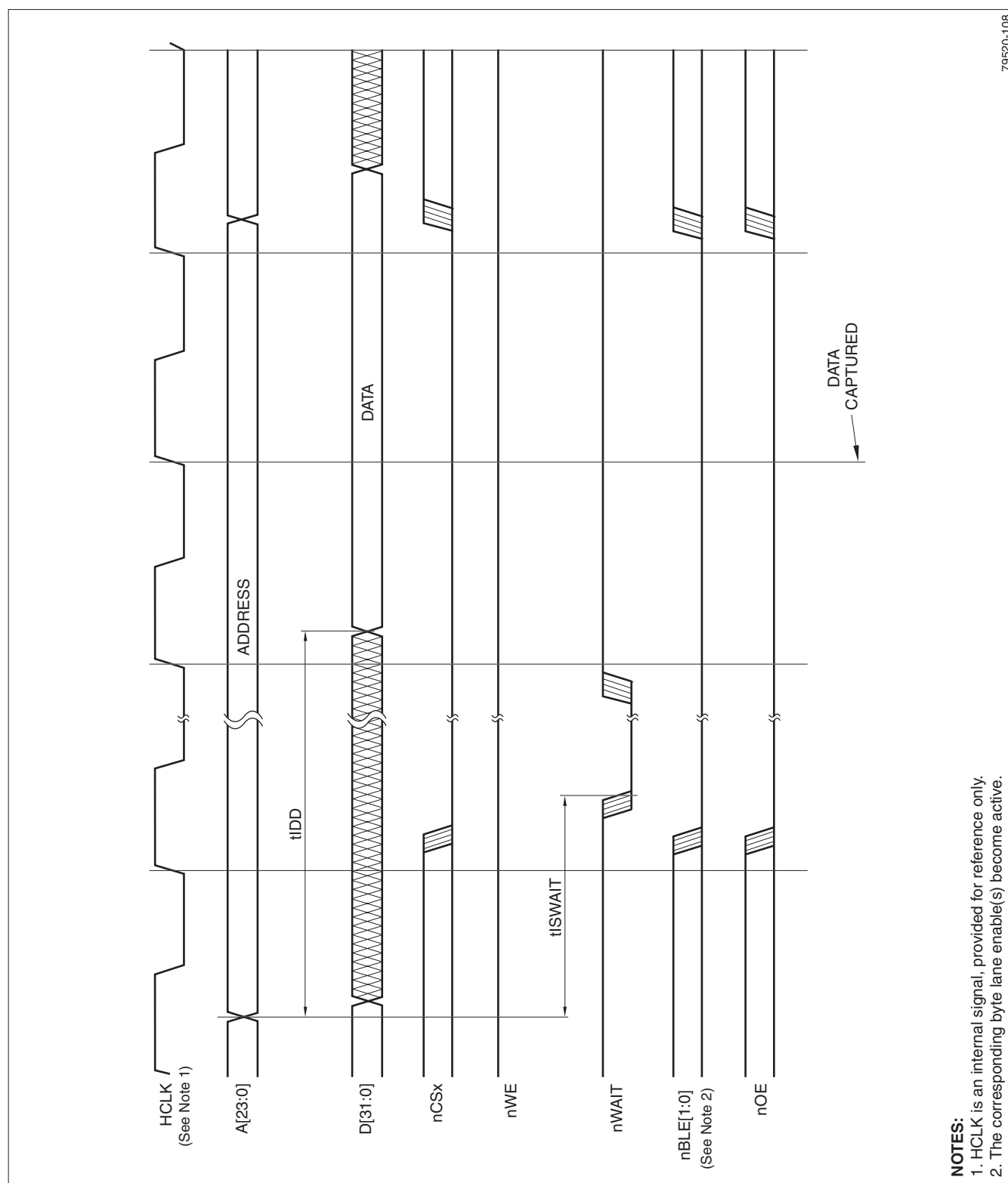
Figure 11. nWait Assertion
