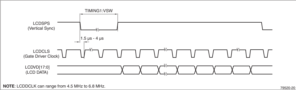
Figure 28. AD-TFT and HR-TFT Vertical Timing Diagram
