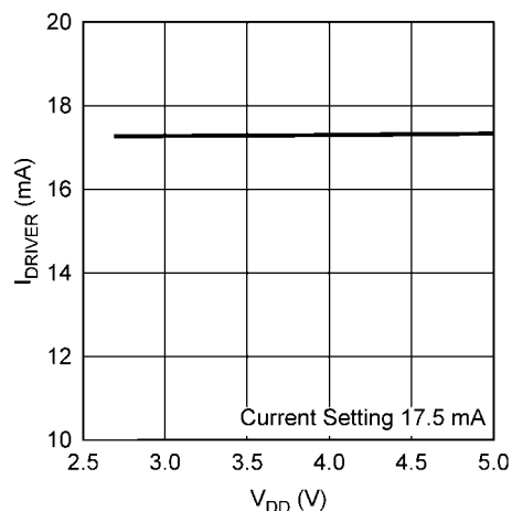
LED Current vs. Supply Voltage
