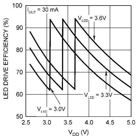
LED Drive Efficiency vs. Input Voltage Automatic Gain Change
