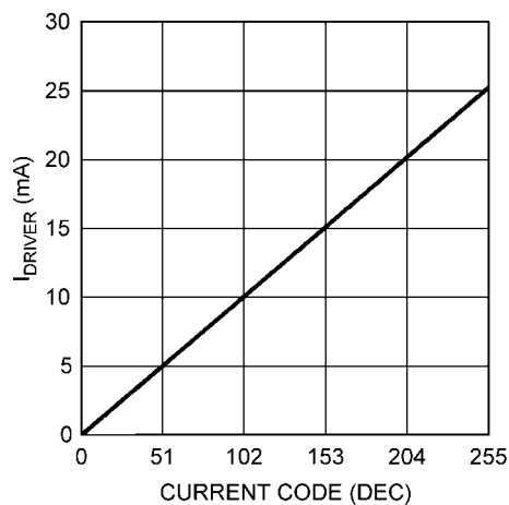
LED Current vs. Current Register Code
