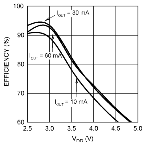
Charge Pump Efficiency vs. Input Voltage 1.5x Mode
