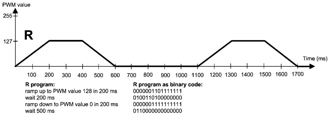
Sequence diagram
