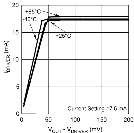
LED Current vs. Output Pin Headroom Voltage
