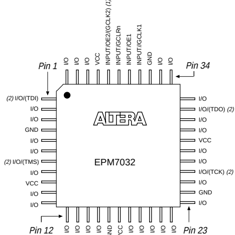
44-Pin PQFP
