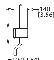
SMT, -M89 Modification Code
