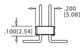
SMT, -M30 Modification Code
