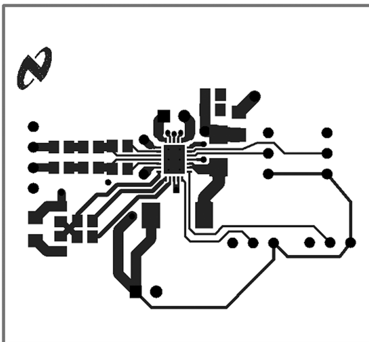
Figure 4. Top Layer
