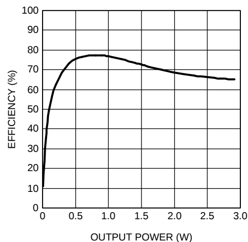
Boost Amplifier vs Output Power
