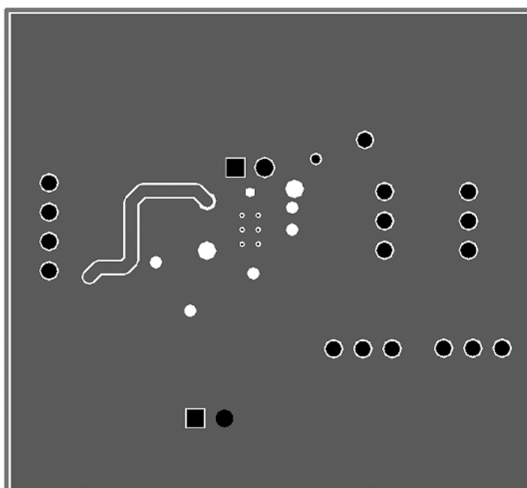
Figure 6. Mid Layer 2
