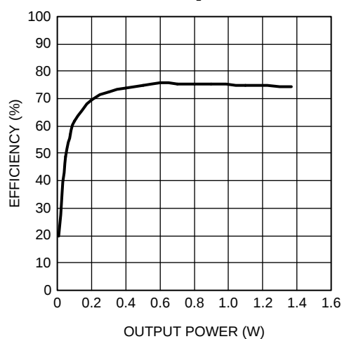
Boost Amplifier vs Output Power
