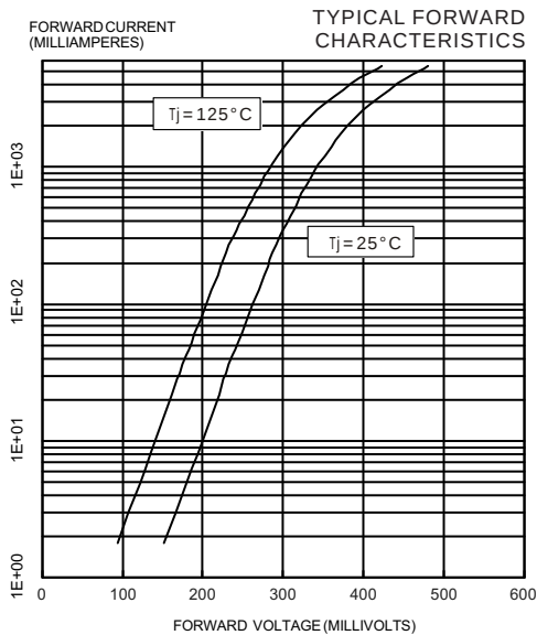
FIG. 7 (For CDBA340L)
