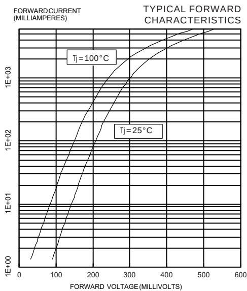
FIG. 8 (For CDBA340LL)
