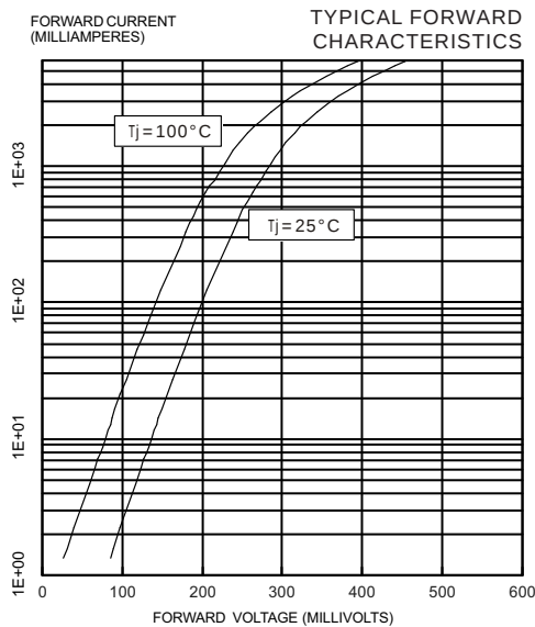
FIG. 6 (For CDBA320LL)
