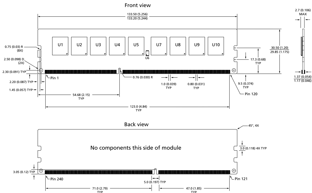
Figure 6: 240-Pin DDR3 UDIMM – PCB 1483
