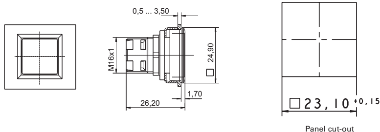
Panel cut-out
