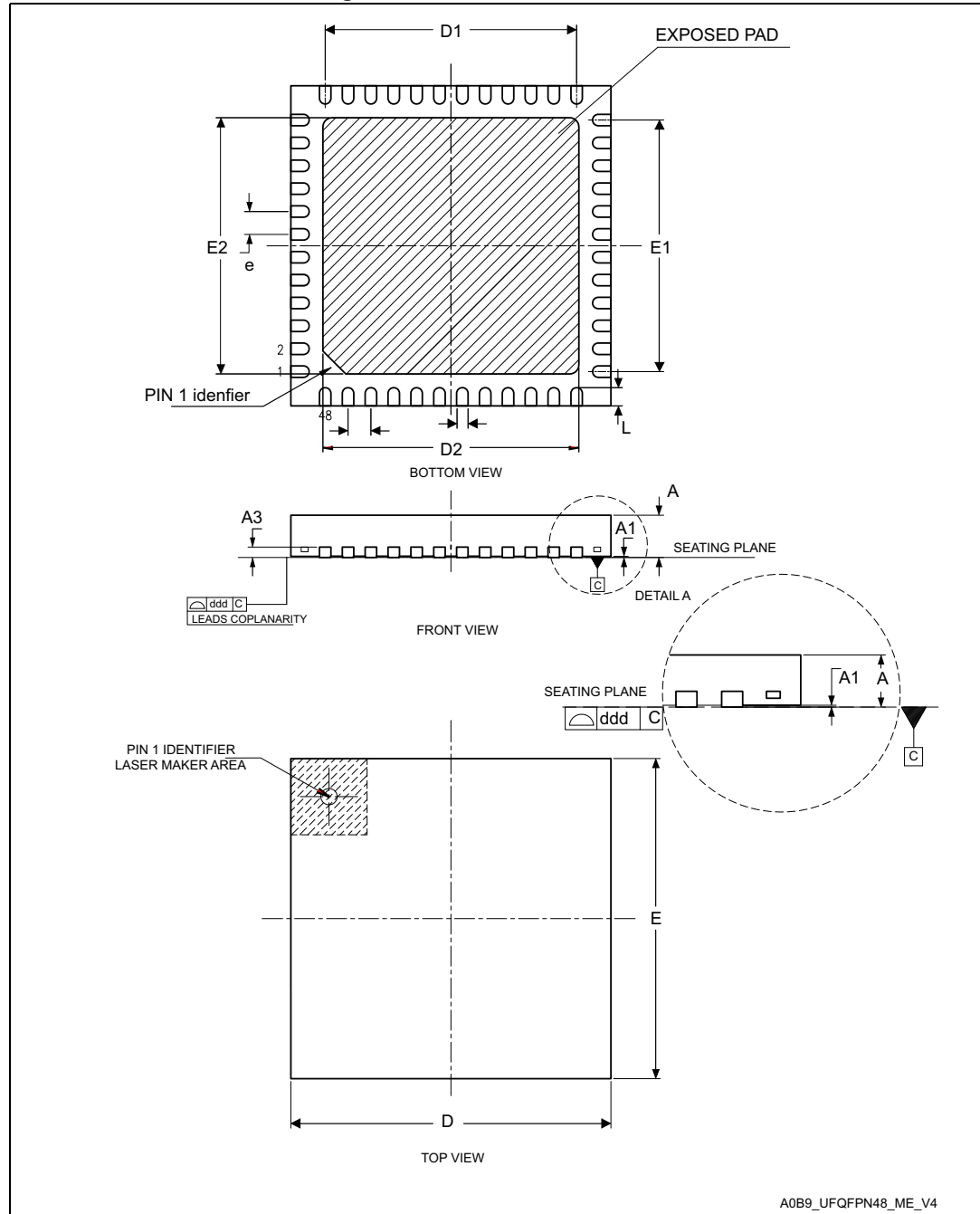
Figure 46. UFQFPN48 – Outline
