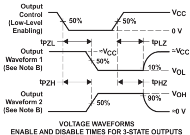
Figure 7-1. Load Circuit and Voltage Waveforms
