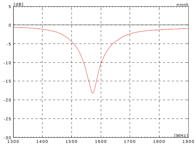
Reference Board A10204-U1
