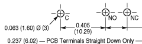
PCB Terminal Footprint
