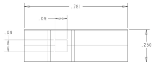
PCB Terminal Footprint
