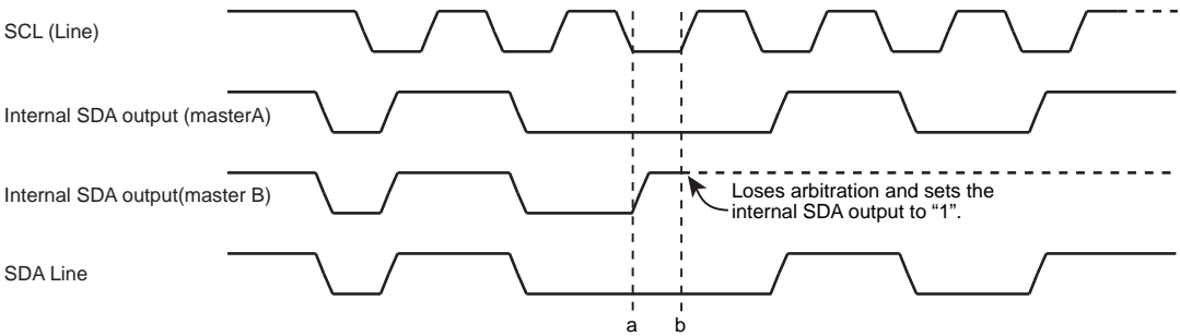
Figure 11-7 Lost Arbitration
