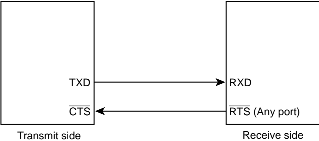
Figure 10-8 Handshake Function
