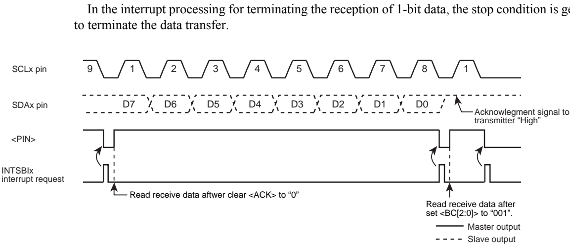
Figure 11-12 Terminating Data Transmission in the Master Receiver Mode
