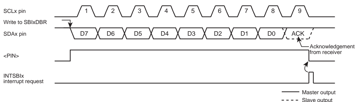
Figure 11-10 &lt;BC[2:0]&gt;= "000", &lt;ACK&gt;= "1" (Transmitter Mode)
