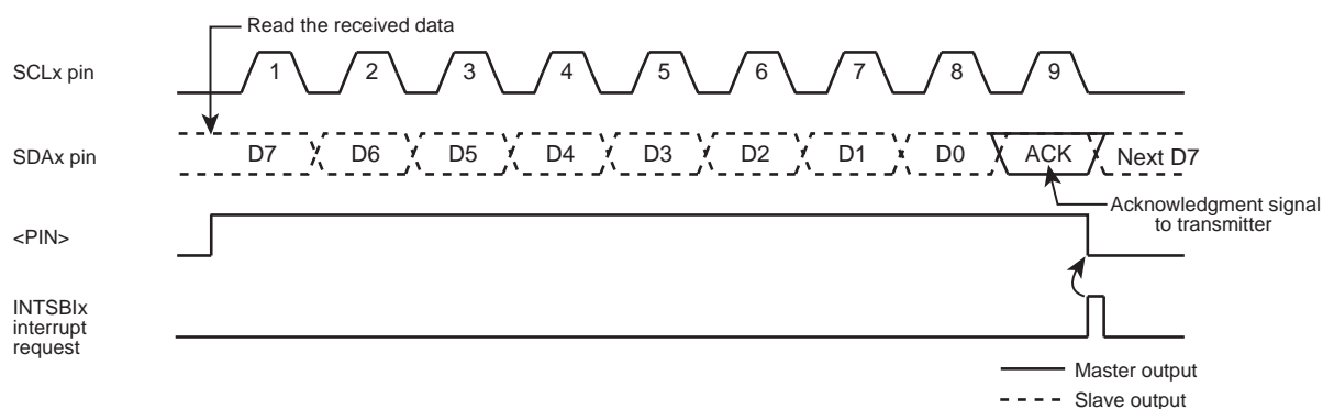
Figure 11-11 &lt;BC[2:0]&gt;= "000", &lt;ACK&gt;= "1" (Receiver Mode)
