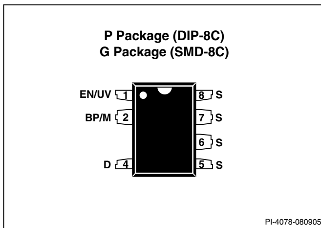
Figure 3. Pin Configuration.
