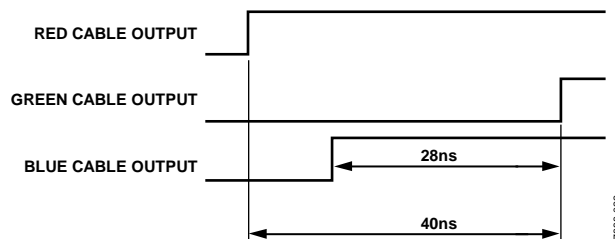
Figure 16. Cable Delay Example
