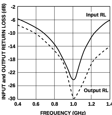
Figure 13. Input and Output Return Loss Results.
