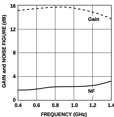
Figure 12. Gain and Noise Figure Results.
