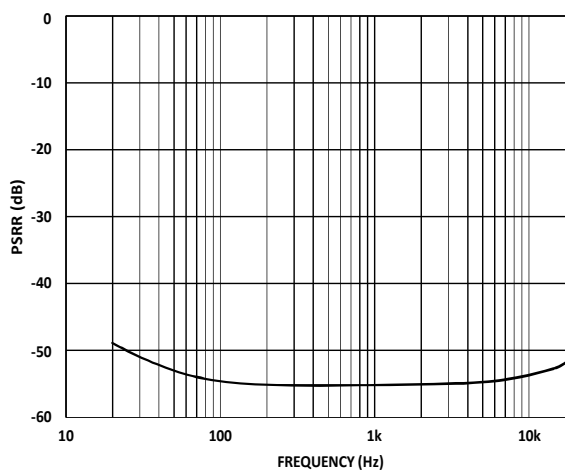
Figure 8. Power Supply Rejection Ratio vs. Frequency
