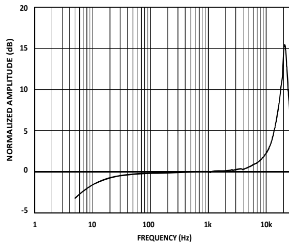
Figure 4. Frequency Response (Measured)
