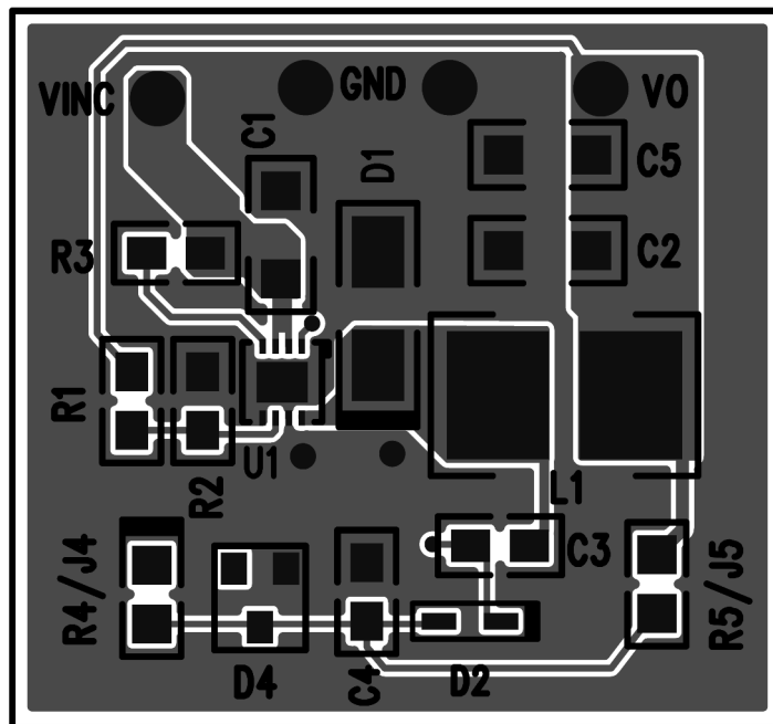
Figure 3-1. Top Layer
