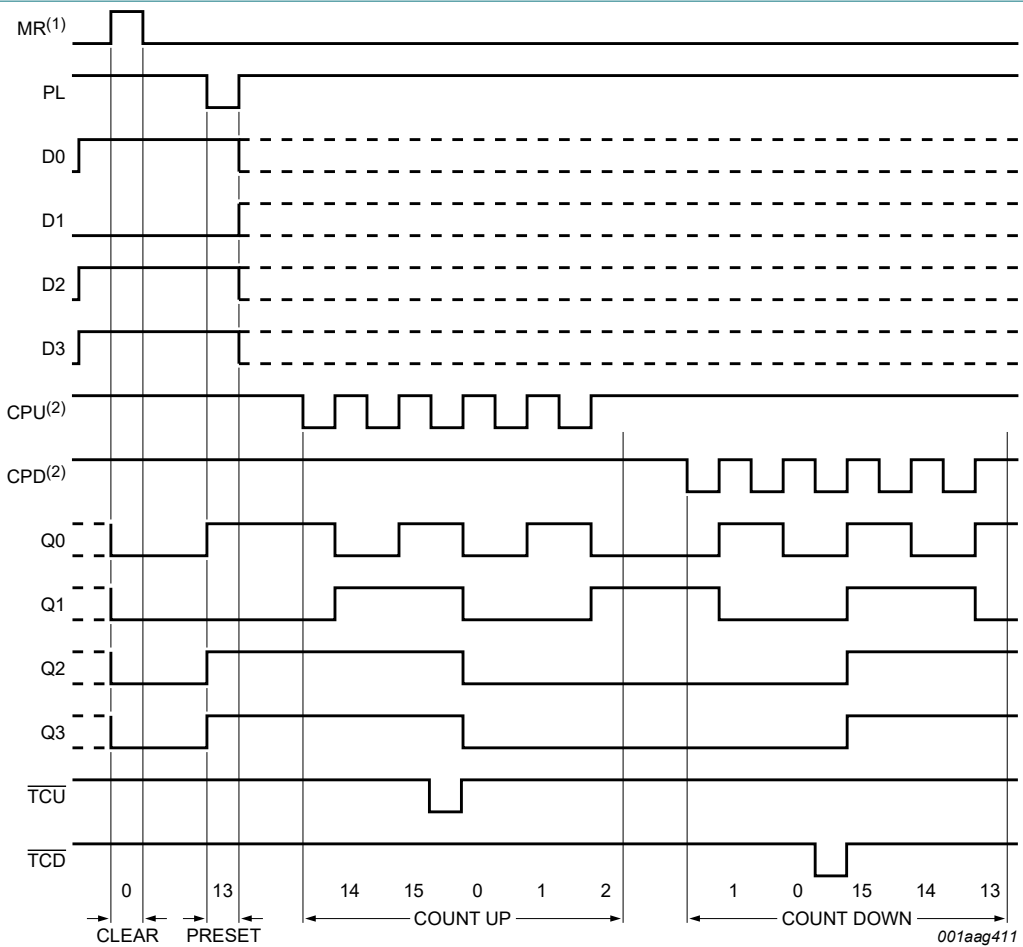
(1) Clear overrides load, data and count inputs. (2) When counting up, the count down clock input (CPD) must be HIGH, when counting down the count up clock input (CPU) must be HIGH. Sequence: Clear (reset outputs to zero); Load (preset) to binary thirteen; Count up to fourteen, fifteen, terminal count up, zero, one and two; Count down to one, zero, terminal count down, fifteen, fourteen and thirteen.
