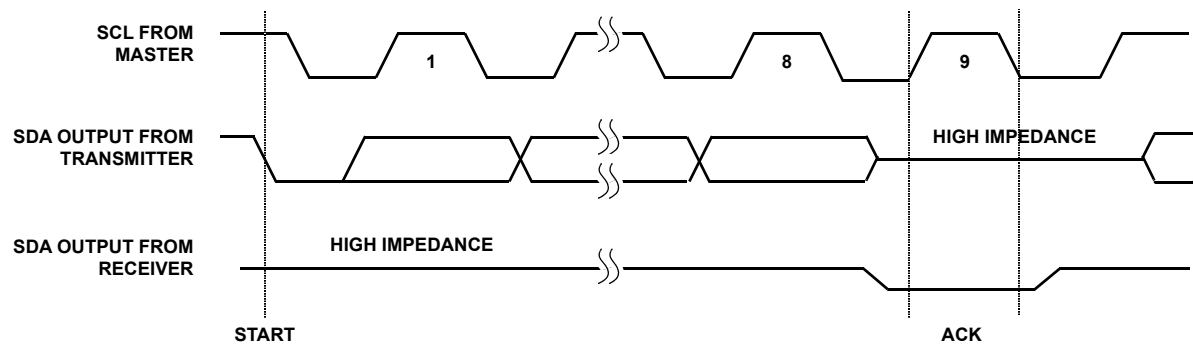
FIGURE 21. ACKNOWLEDGE RESPONSE FROM RECEIVER
