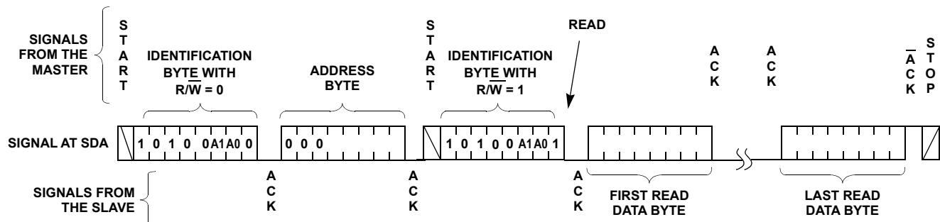
FIGURE 23. READ SEQUENCE
