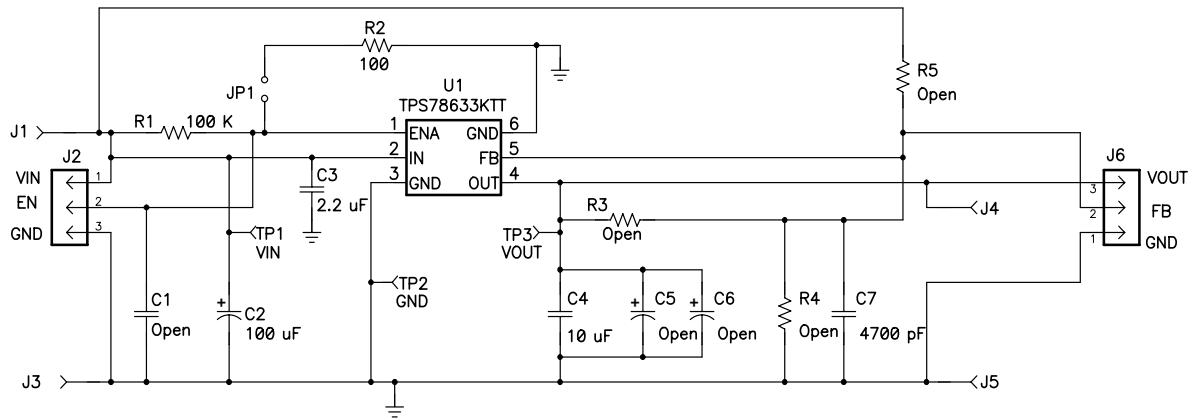
Figure 4–1. Schematic
