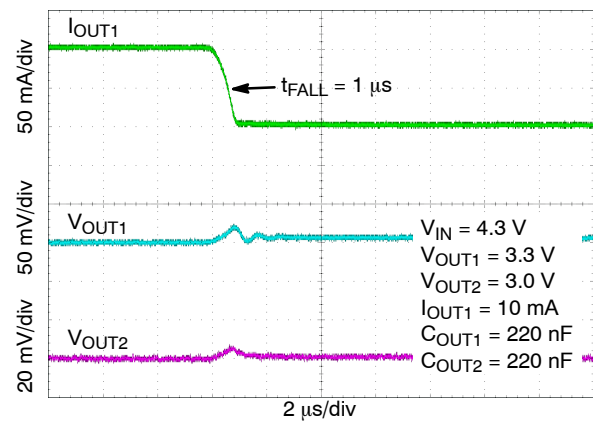
Figure 51. Load Transient Response – Falling Edge, I_{OUT} = 150 mA to 50 mA
