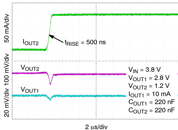
Figure 42. Load Transient Response – Rising Edge, I_{OUT} = 0.1 \text{ mA} to 150 mA
