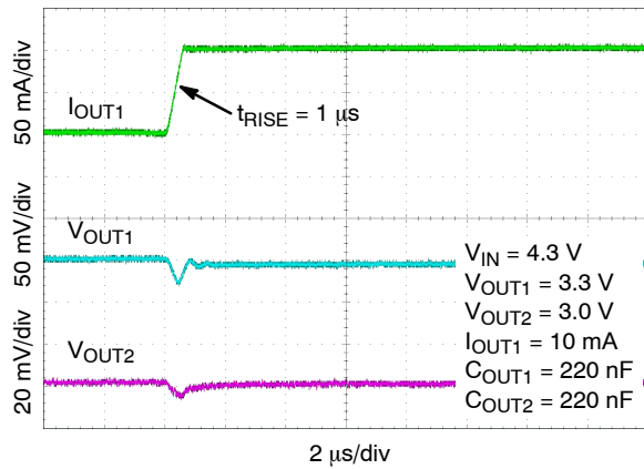
Figure 50. Load Transient Response – Rising Edge, I_{OUT} = 50 mA to 150 mA
