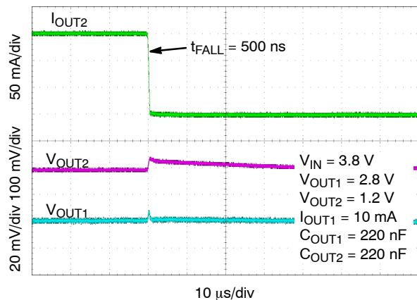
Figure 43. Load Transient Response – Falling Edge, I_{OUT} = 150 \text{ mA} to 0.1 mA
