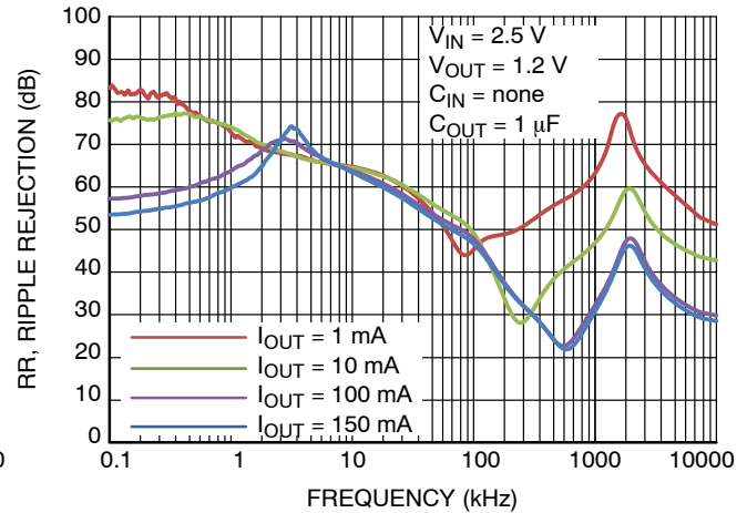
Figure 24. Power Supply Rejection Ratio, V_{OUT} = 1.2\text{ V} , C_{OUT} = 1\text{ }\mu\text{F}
