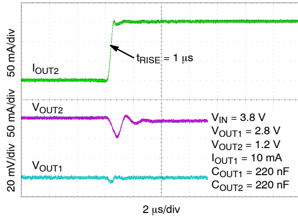
Figure 40. Load Transient Response – Rising Edge, I_{OUT} = 1 \text{ mA} to 150 mA
