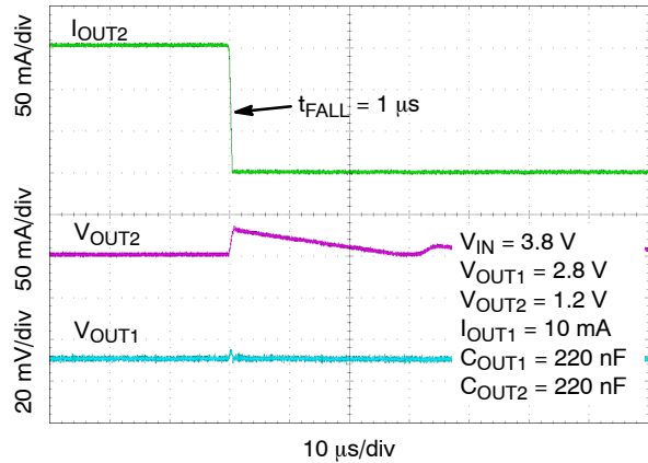
Figure 41. Load Transient Response – Falling Edge, I_{OUT} = 150 \text{ mA} to 1 mA
