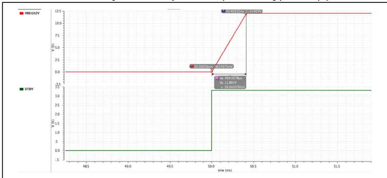
Figure 11: "Standby to normal" operation timing (C REG = 1 µF)
