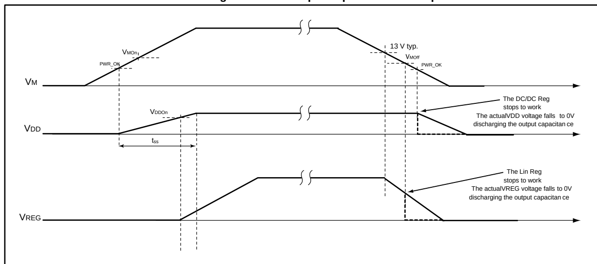
Figure 6: Power-up and power-down sequence
