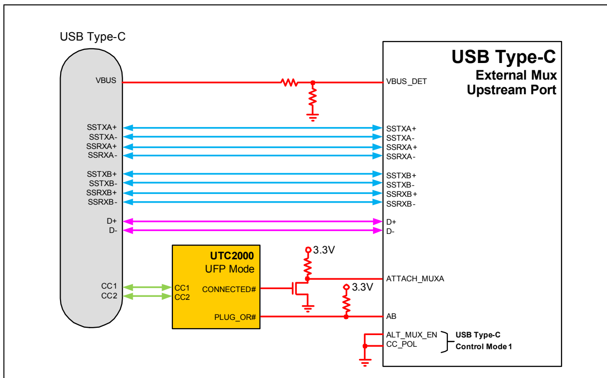
FIGURE 8-2: UFP TYPE-C PORT WITH MICROCHIP UTC2000 & EXTERNAL MUX (MODE 1)
