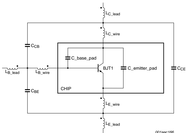
Fig 9. Package equivalent circuit of SOT343R
